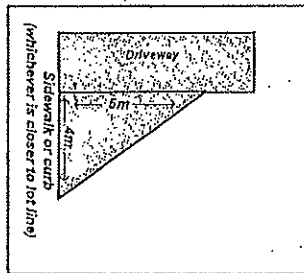
1.07 metres (3 feet, 6 inches) in General Driveway Sight Line Triangle Detail
